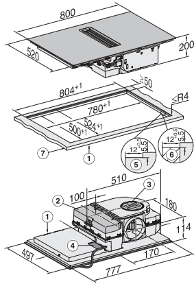
KMDA7272FL, KMDA7473FL – flush – Installation drawing
